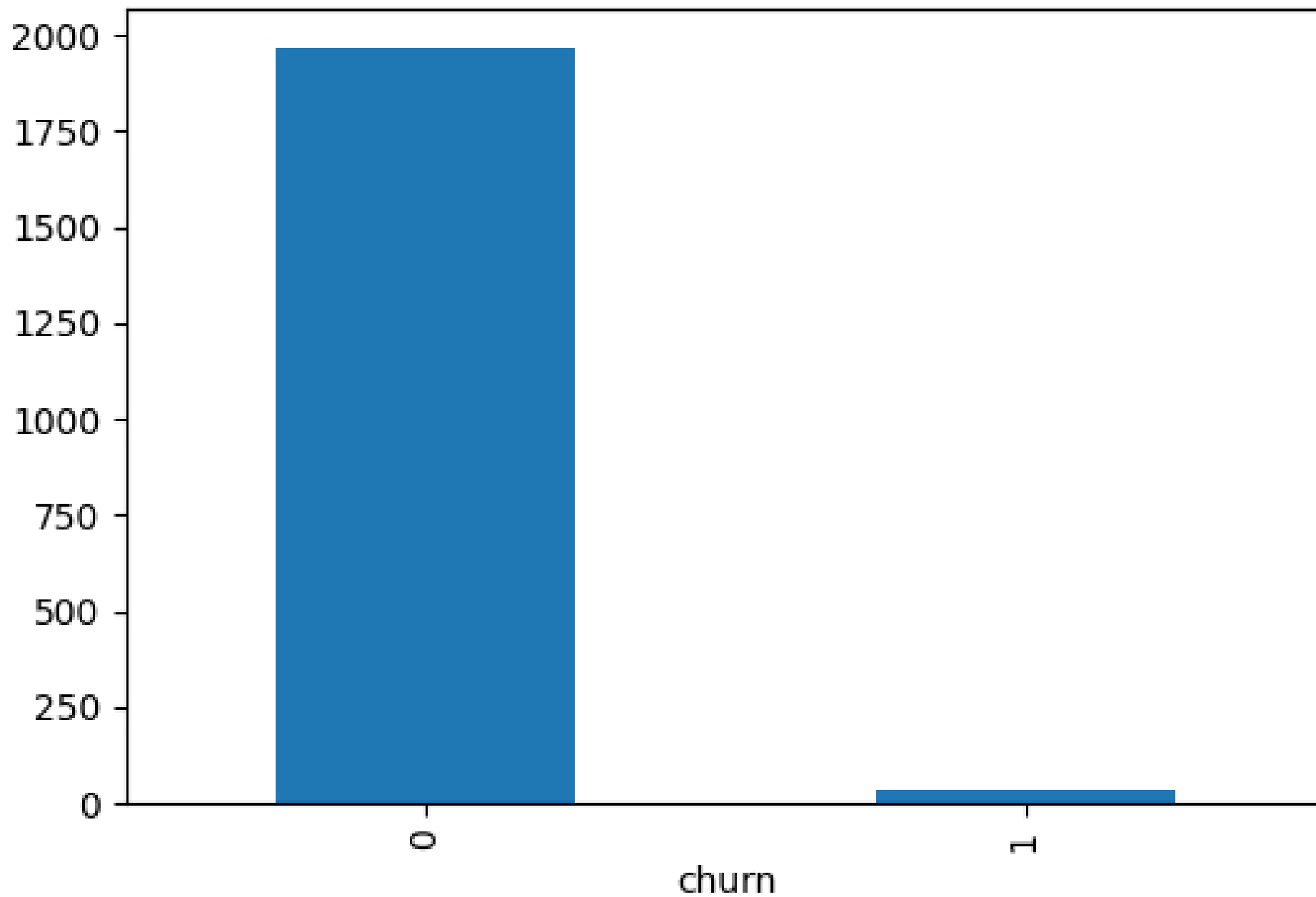
Churn Distribution
