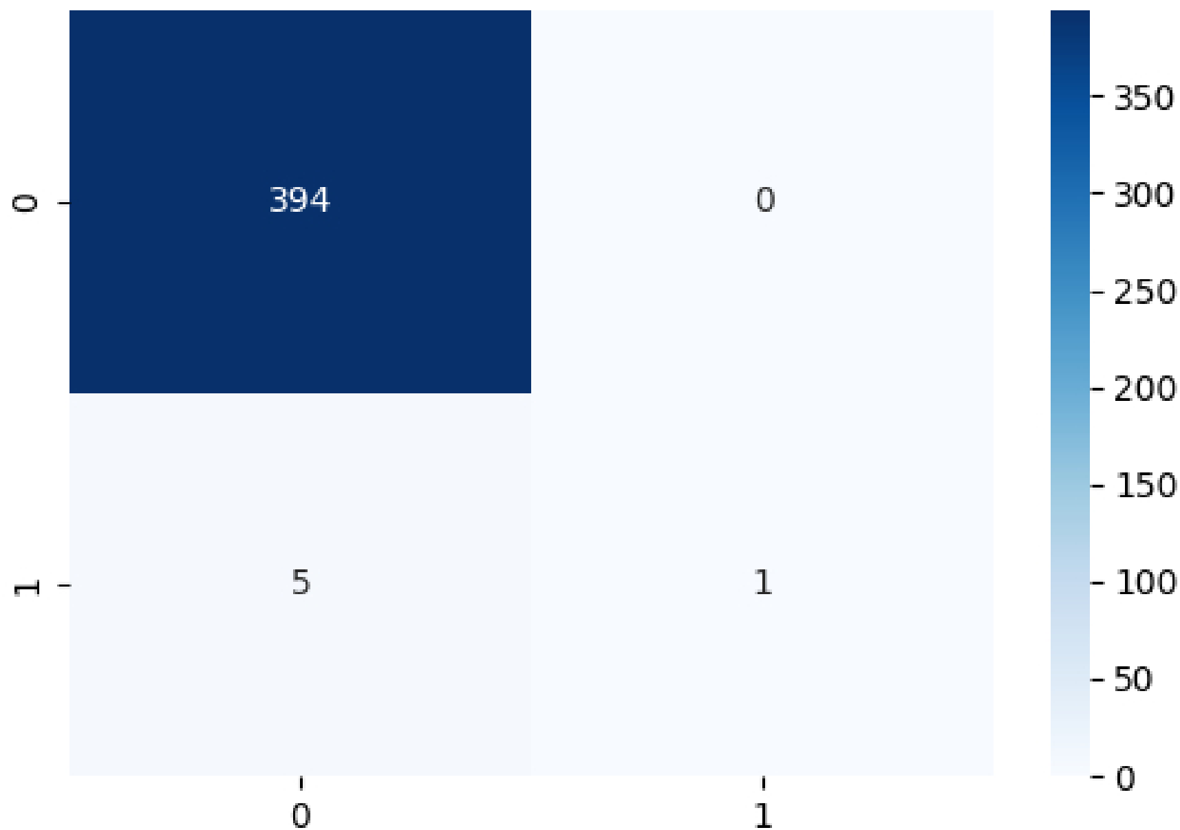
Confusion Matrix
