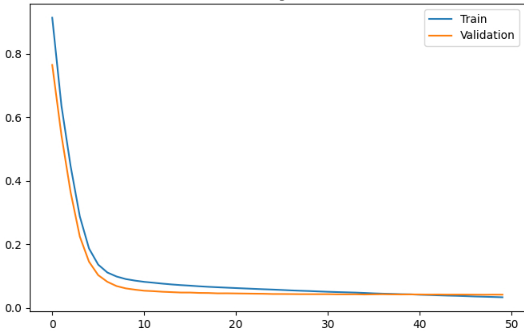
Training Loss
